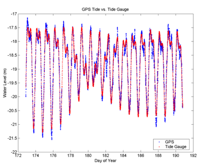
Fig. 4. CHS tide gauge data (red) and NAVOCEANO's P&TB data (blue)
