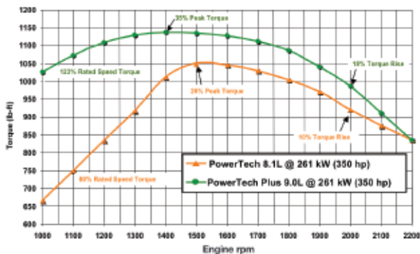
Tier 3/Stage III A PowerTech Plus 9.0L vs. Tier 2/Stage II A PowerTech 8.1L
