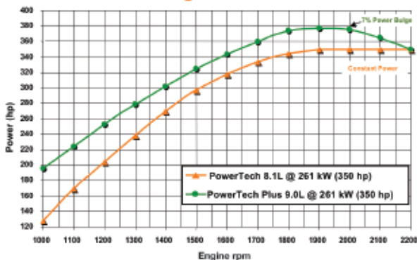
Tier 3/Stage III A PowerTech Plus 9.0L vs. Tier 2/Stage II PowerTech 8.1L
