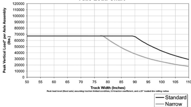
Axle Load Chart
